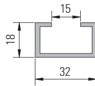
AP-4 Article no. 209580 (max. length 6 m)
