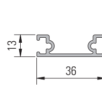
AP-G1 Article no. 209596 (max. length 6 m)
